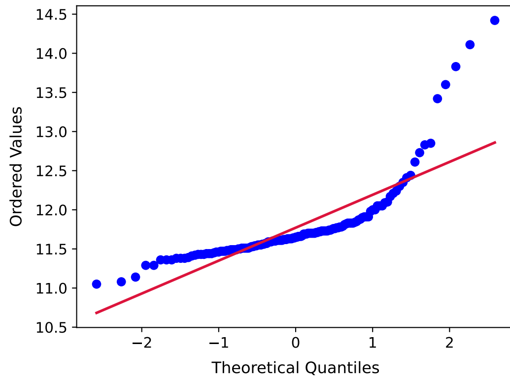
Mahalanobis Q-Q Plot
