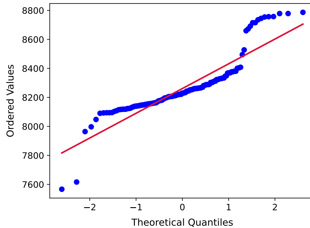
SAM2 Q-Q Plot
